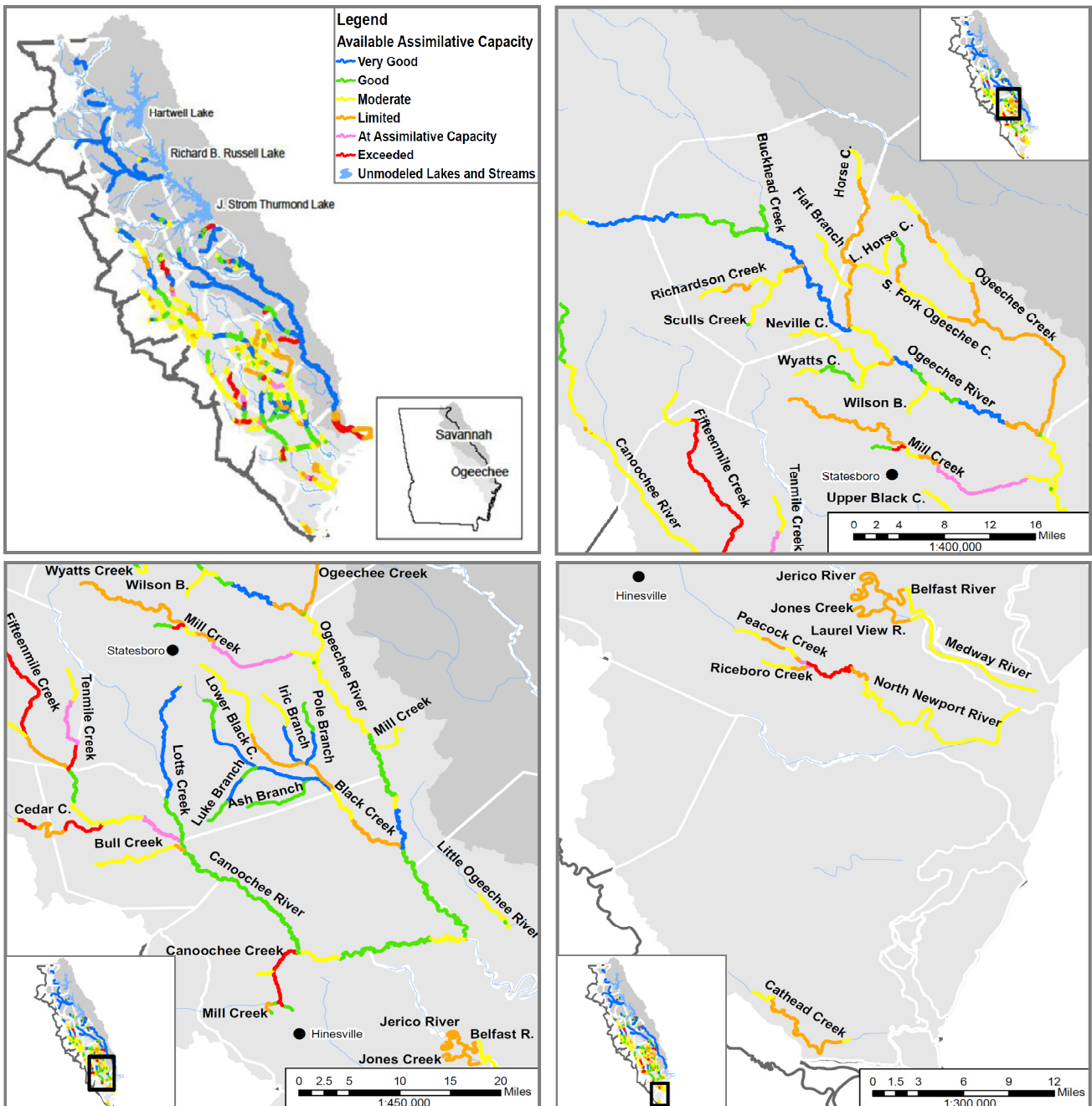
Figure 3-6a: Results of Assimilative Capacity Assessment – DO at Baseline Conditions (Savannah and Ogeechee River Basins)
