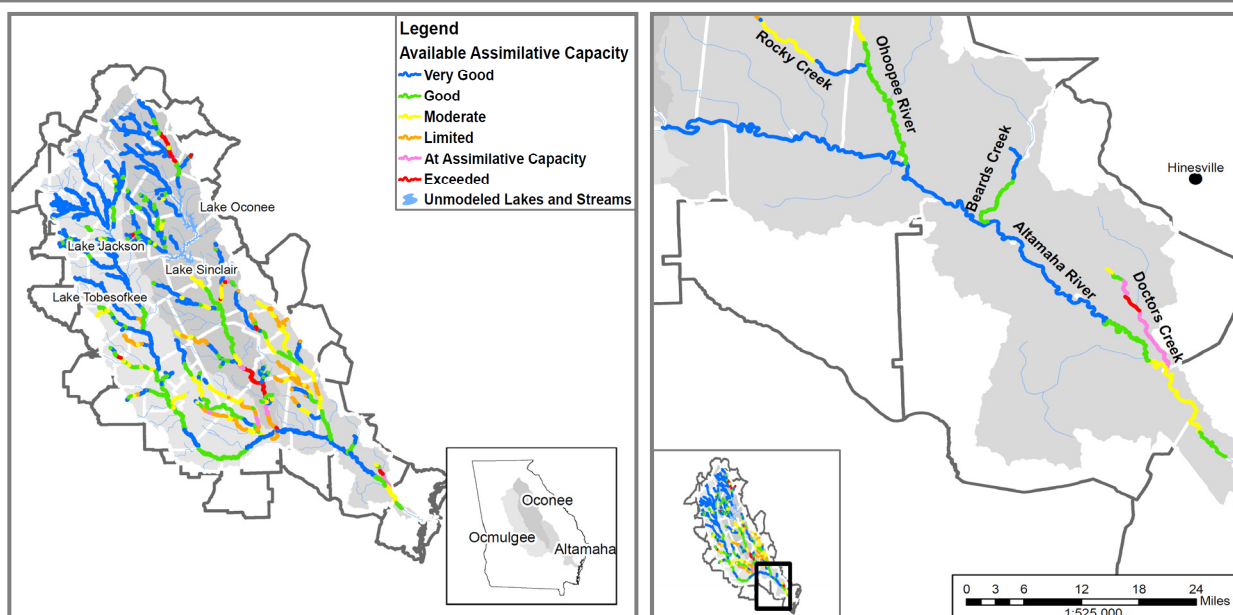
Figure 3-6b: Results of Assimilative Capacity Assessment – DO at Baseline Conditions (Oconee, Ocmulgee, and Altamaha River Basins)
