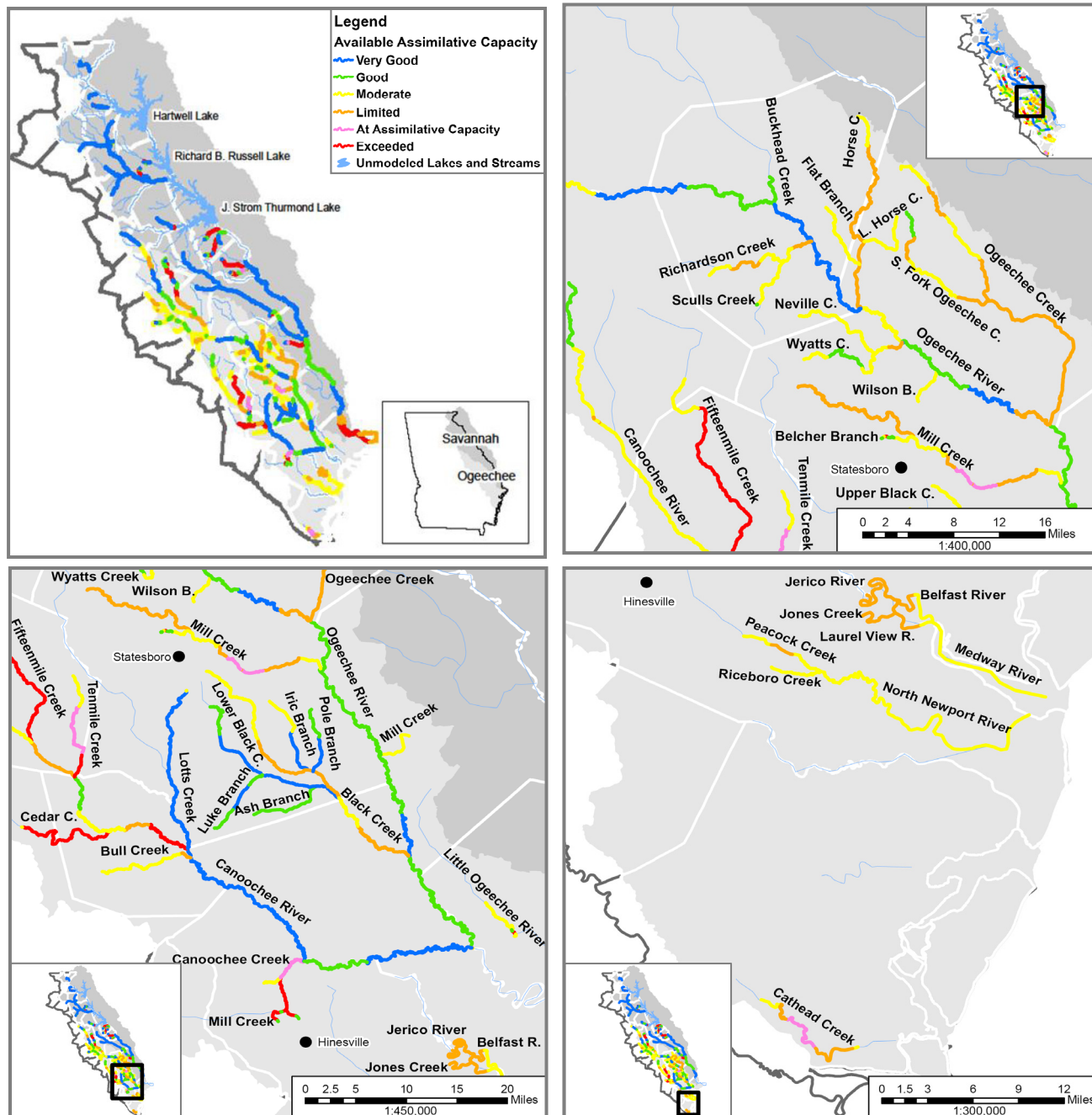
Figure 5-3a: Results of Assimilative Capacity Assessment – DO at Permitted Conditions (Savannah and Ogeechee River Basins)
