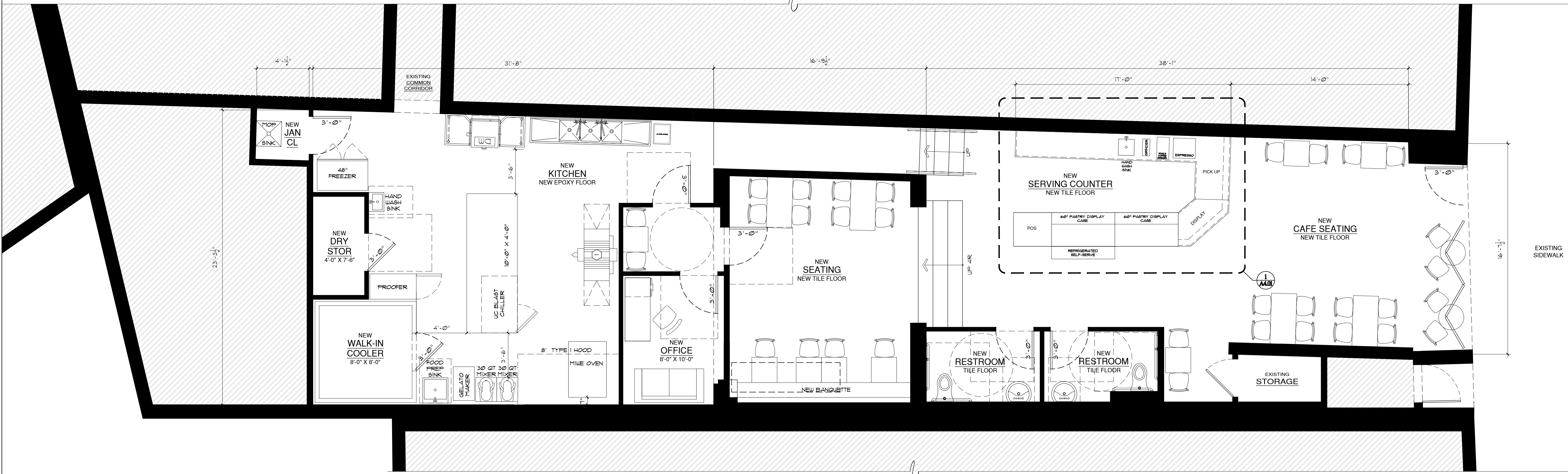
2 New First Floor Architectural Plan (2,085 SF+/- GLA) A1.01 Scale: 1/4" = 1'-0"
