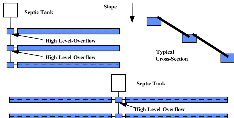
Figure 9 - Serial Distribution Systems
