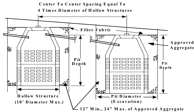
Figure 15 - Leaching Pits
