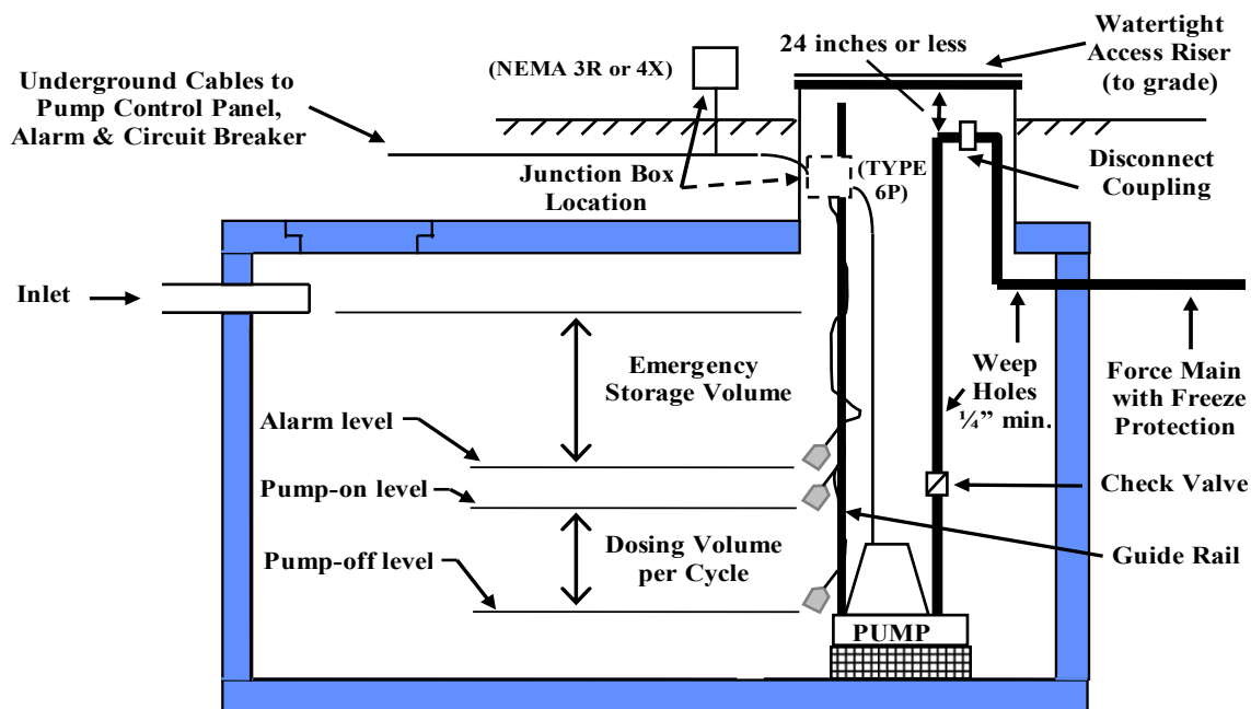
Figure 11 - Pump Chamber
