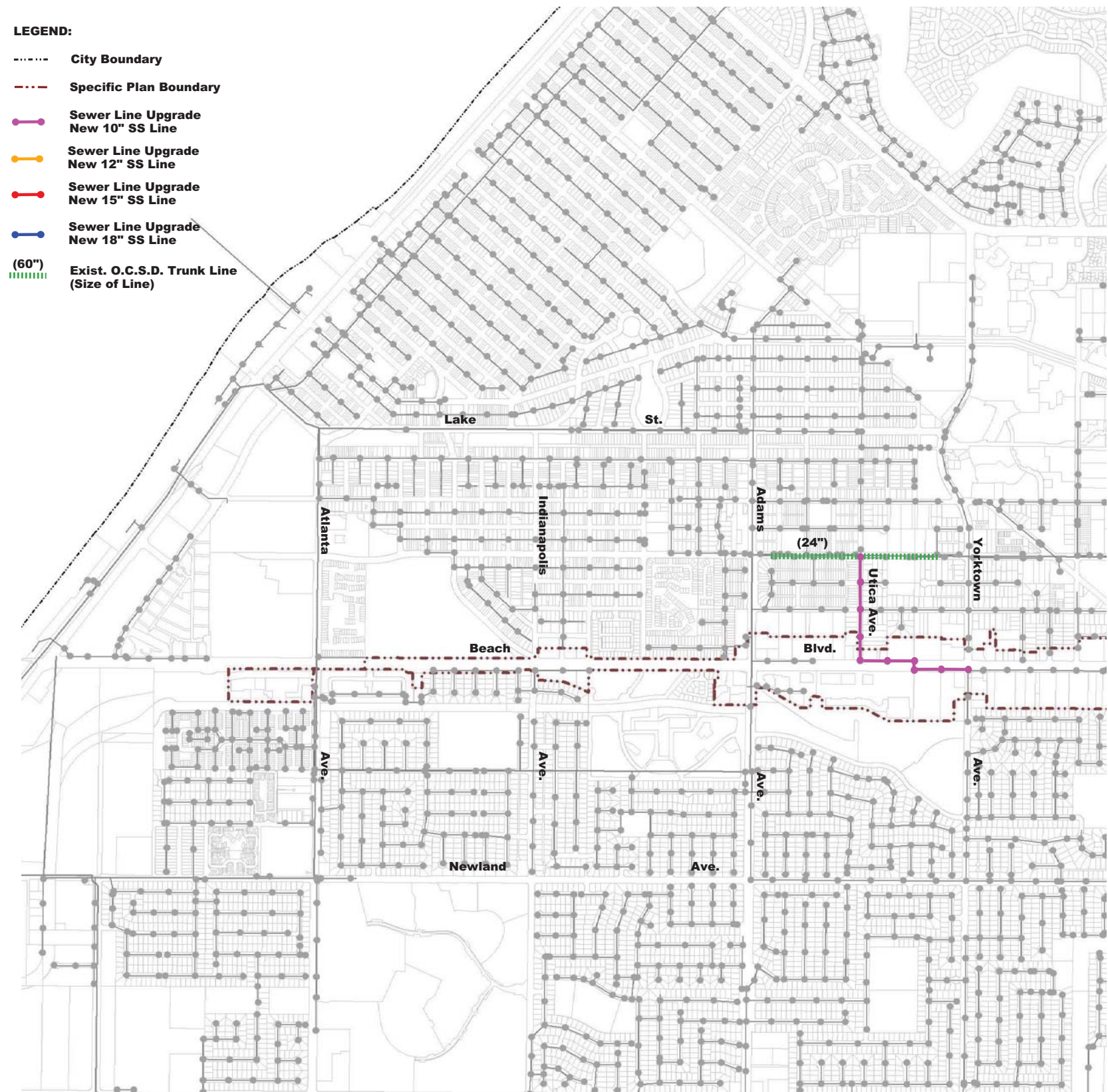
FIG 3.7 WASTEWATER FACILITIES
