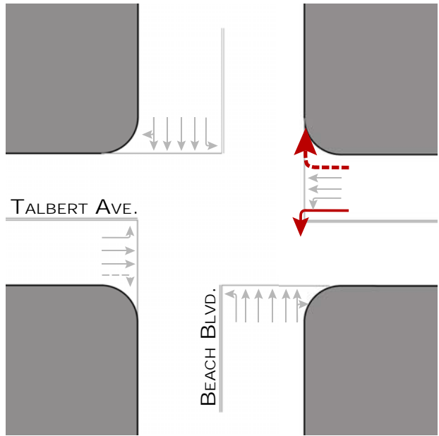
FIG 3.3 BEACH BLVD. & TALBERT AVE. INTERSECTION IMPROVEMENTS
