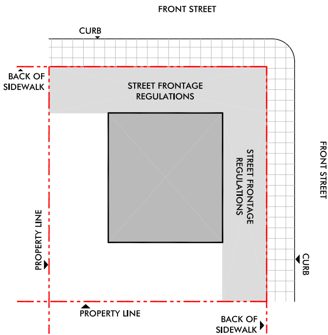
Fig.2.4.2 Private Frontage Types - 2) Corner Parcels
