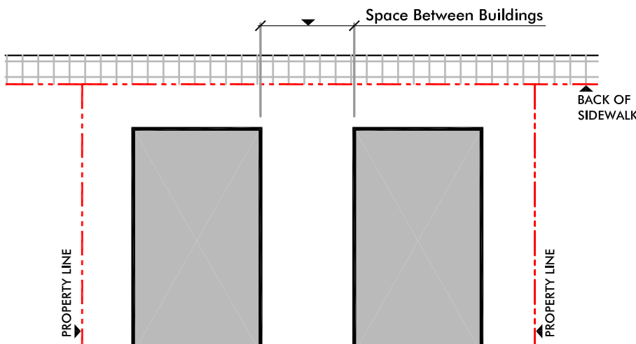
Fig.2.4.8 Space Between Buildings
