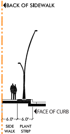
Fig.2.5.1. - 4a) Typical Public Frontage
