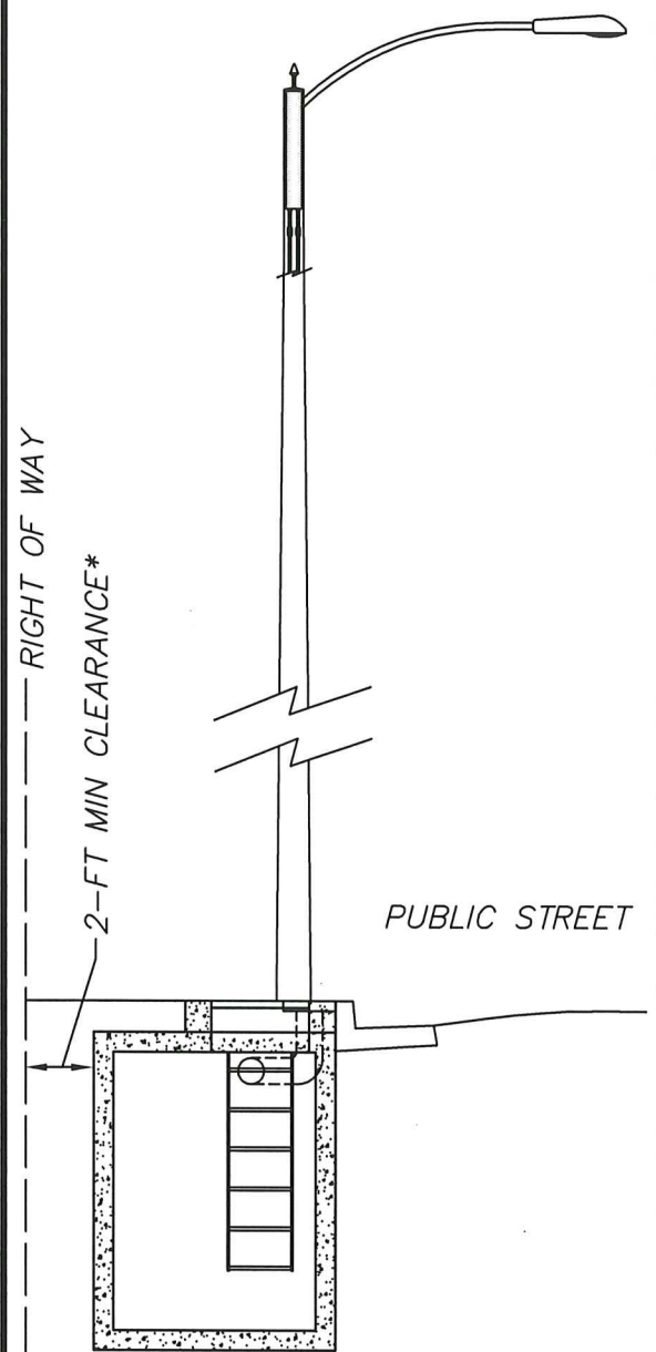
SECTION VIEW
