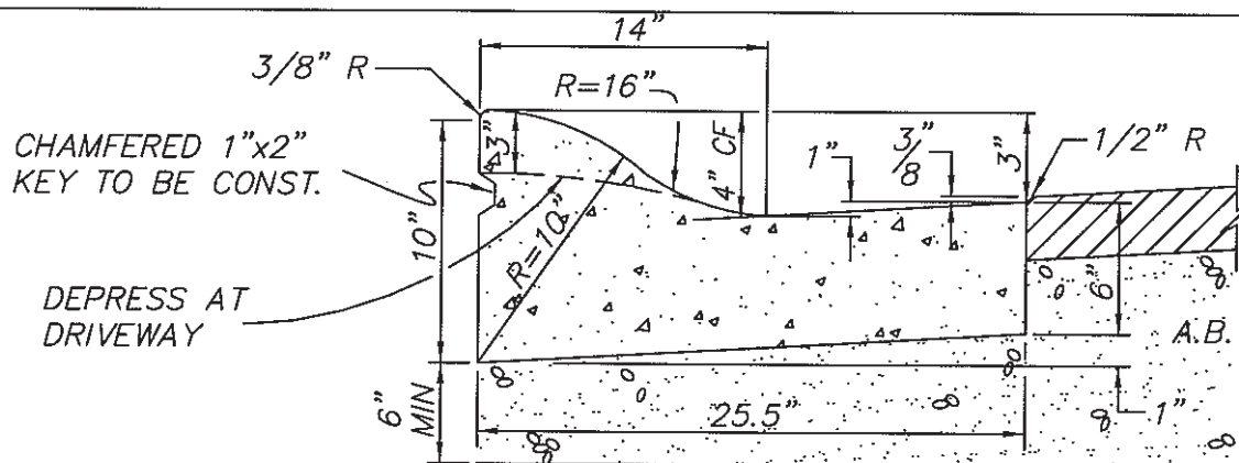
TYP. CONC. ROLLED CURB DETAIL 4" CF
