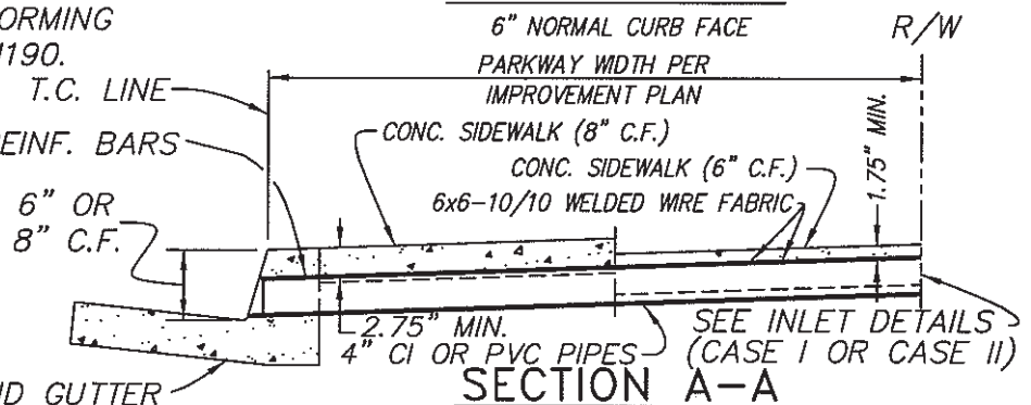
NORMAL CURB PROFILE
