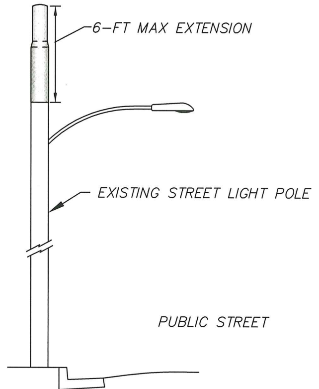
SECTION VIEW
