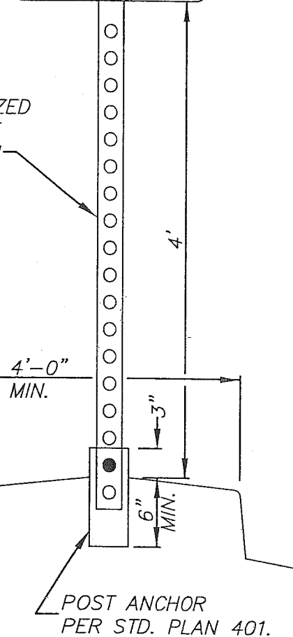
SECTION B-B
