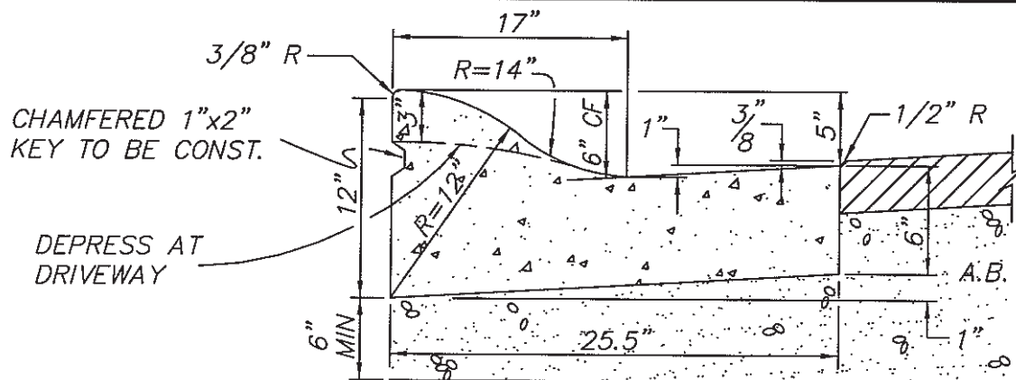
TYP. CONC. ROLLED CURB DETAIL 6" CF
