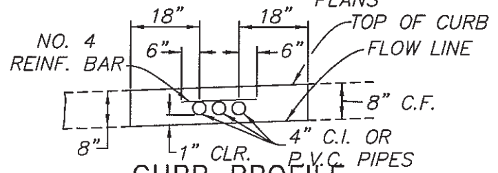
CURB PROFILE
