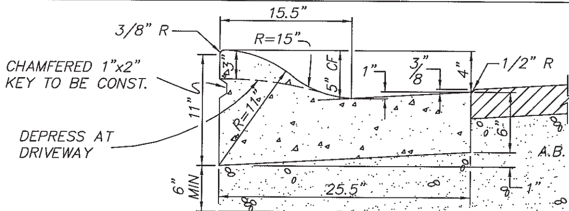
TYP. CONC. ROLLED CURB DETAIL 5" CF
