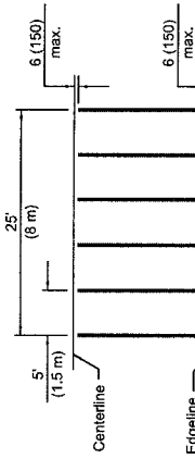
TYPICAL INSTALLATION
