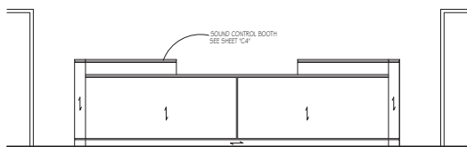
ELEVATION @ "SOUND CONTROL WINDOWS" 1/2" = 1'-0"
