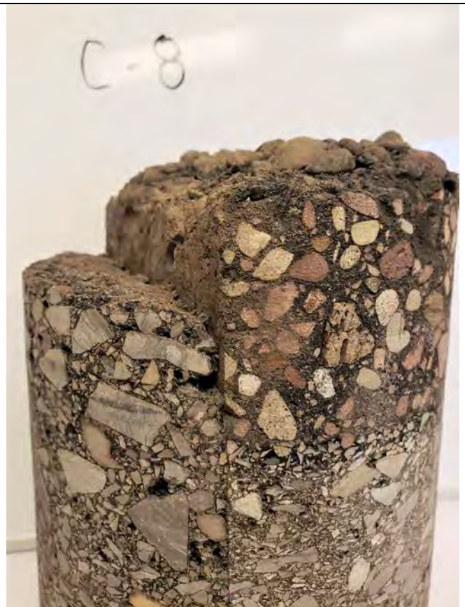
Photograph 10: Core C-8 (Close up view of cut joint)
