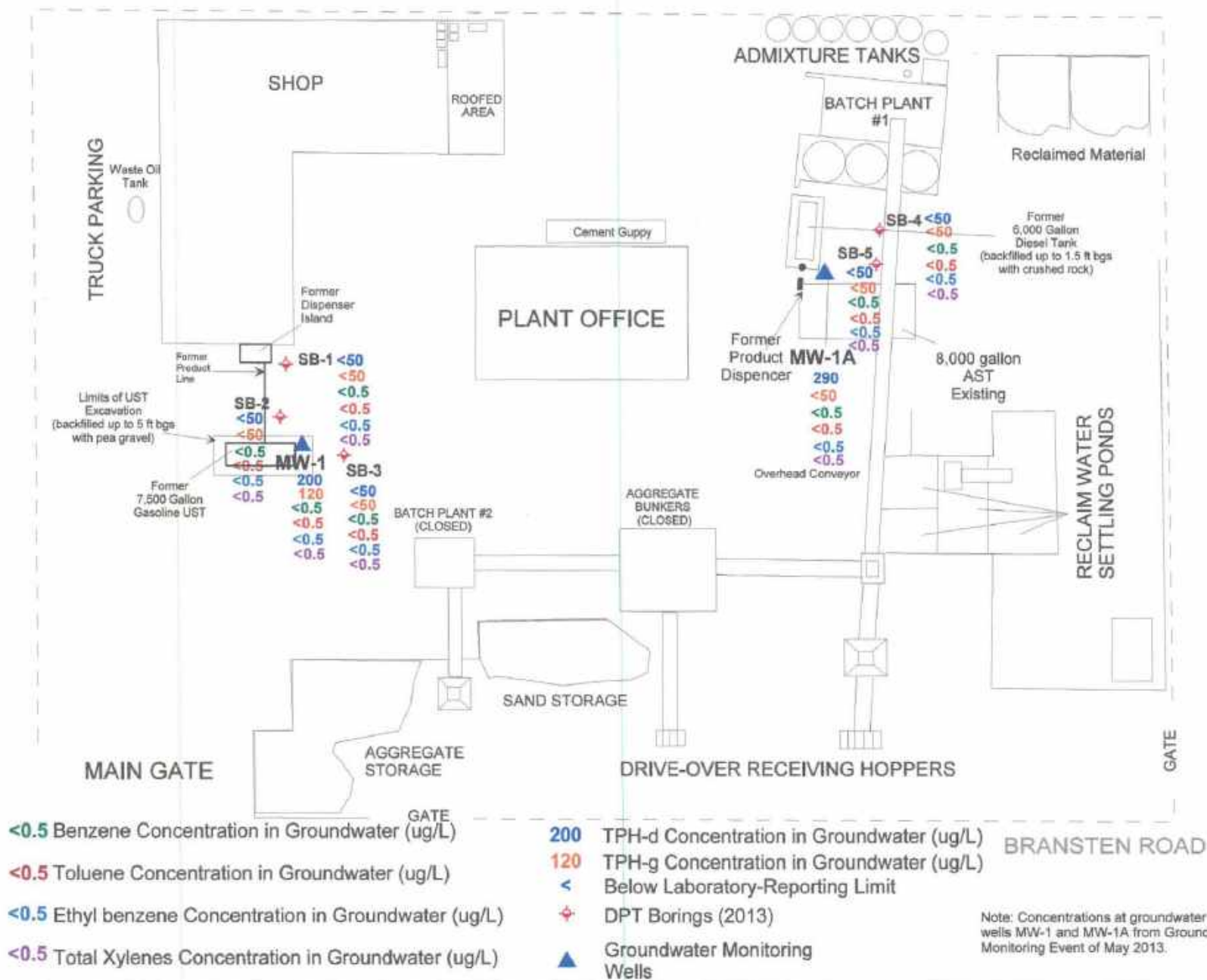
Figure 3: Site Map Showing Chemical Concentrations in Groundwater
