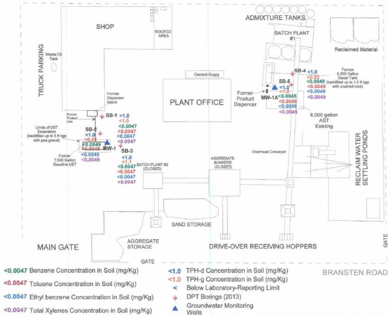
Figure 2: Site Map Showing Concentrations in Soil and Locations of New Borings
