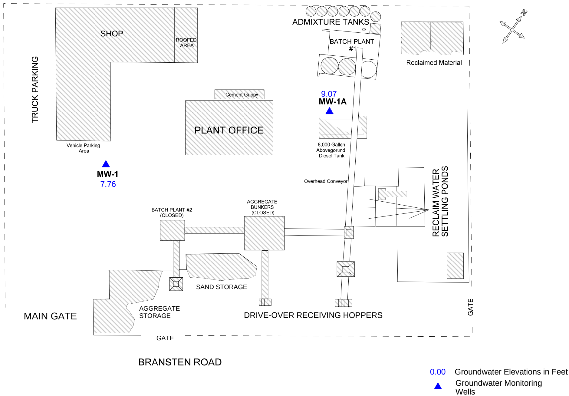
Figure 3: Site Map Showing Groundwater Elevations
