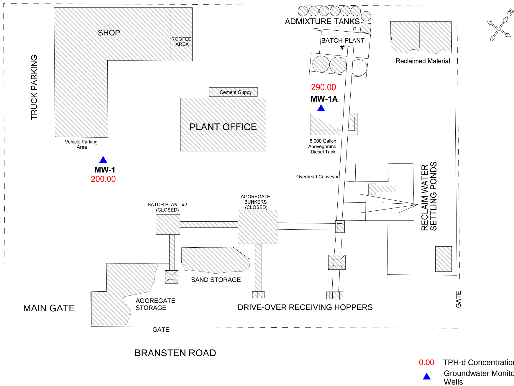
Figure 4: Map Showing TPH-d Concentrations
