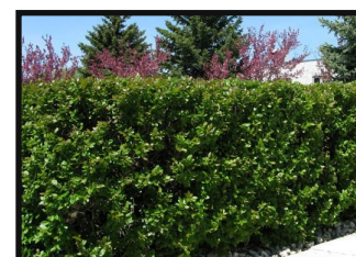
Hedge Cotoneaster
