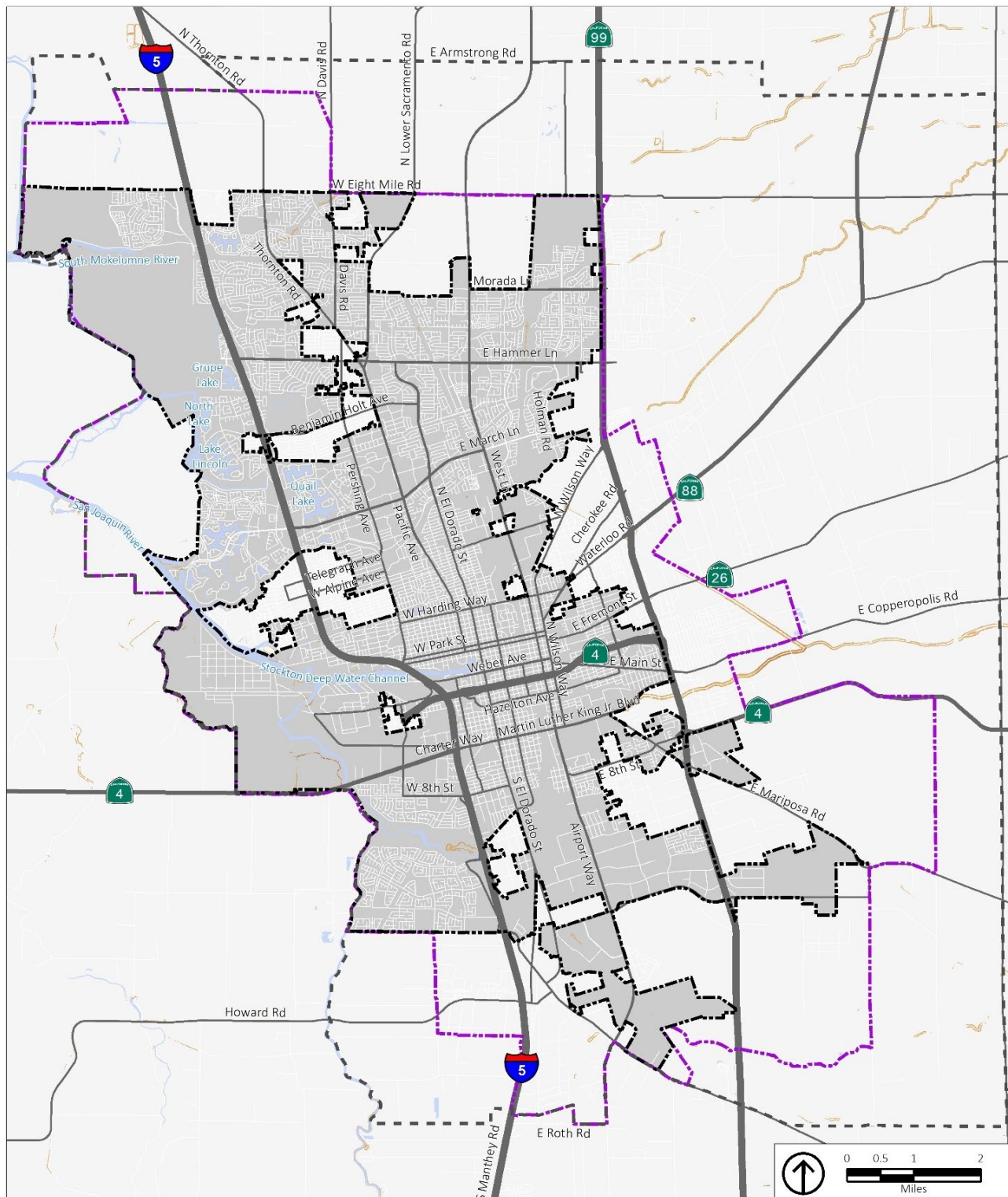
Figure 11 Landslide Susceptibility
