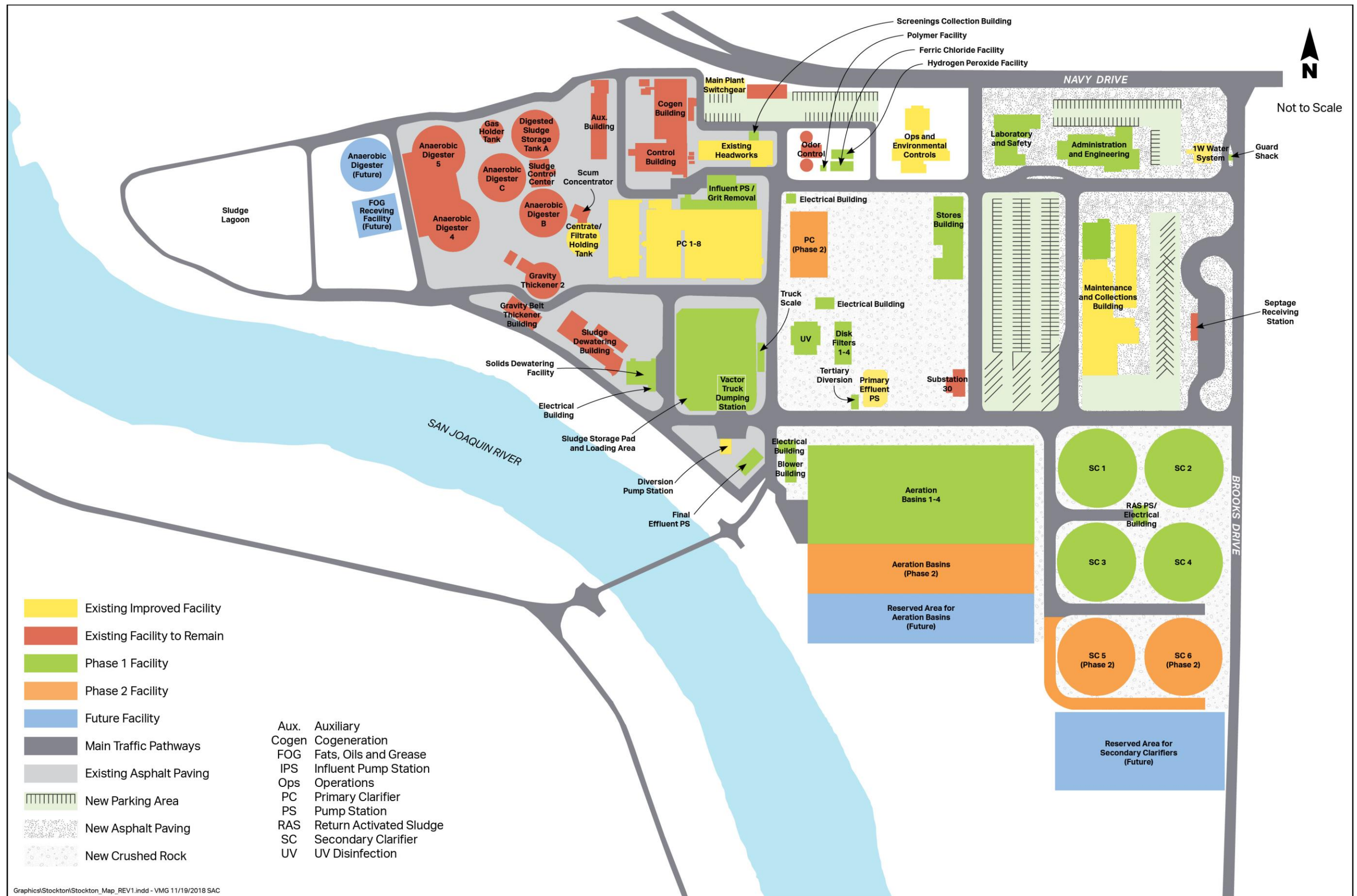
Figure 4-4. City of Stockton RWCF – Proposed Layout
