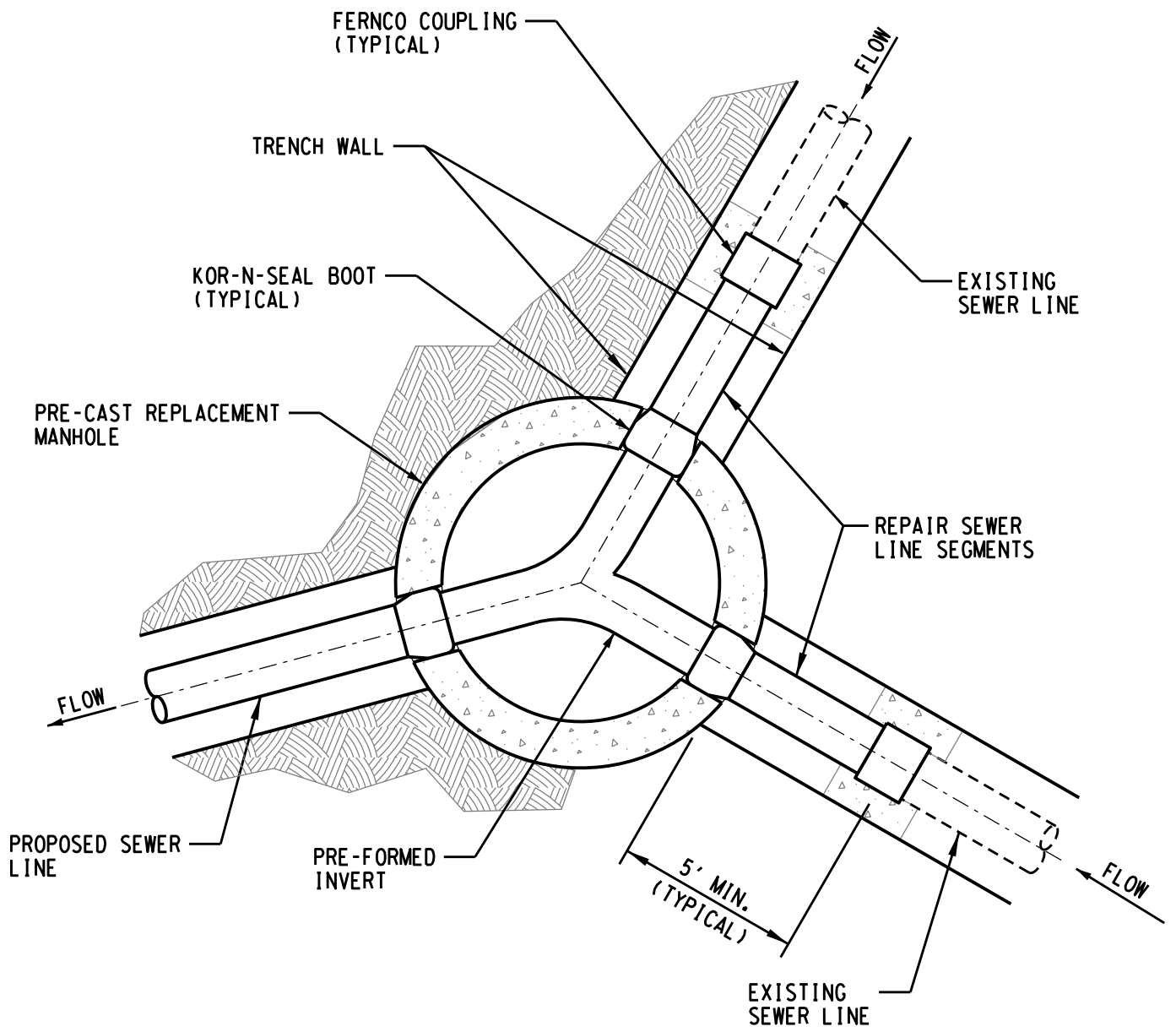
MANHOLE REPLACEMENT DETAIL (CLAY OR CAST IRON)
