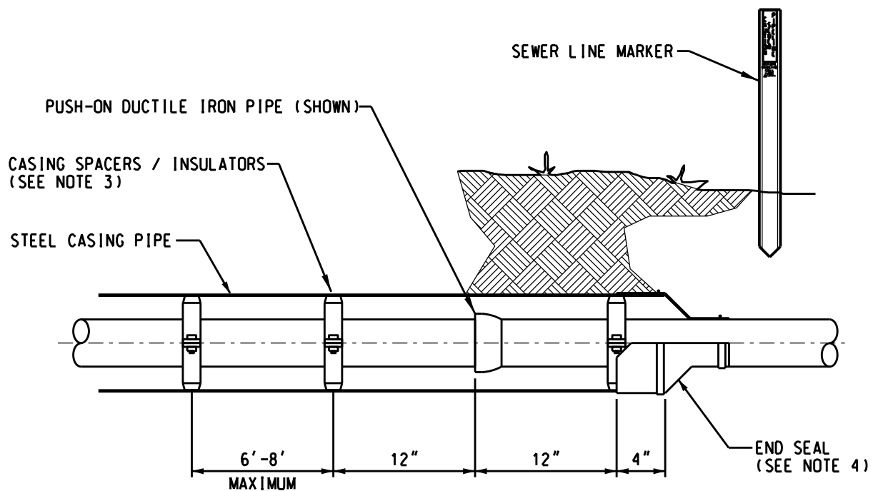
SECTION VIEW
