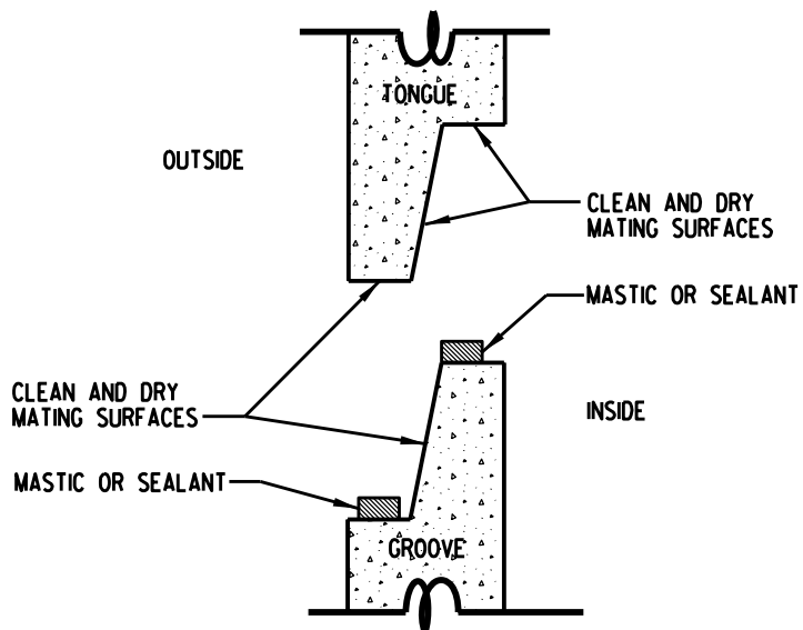
OPEN JOINT
