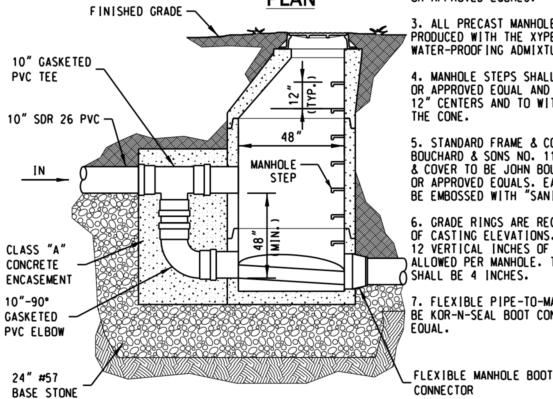
SECTION
