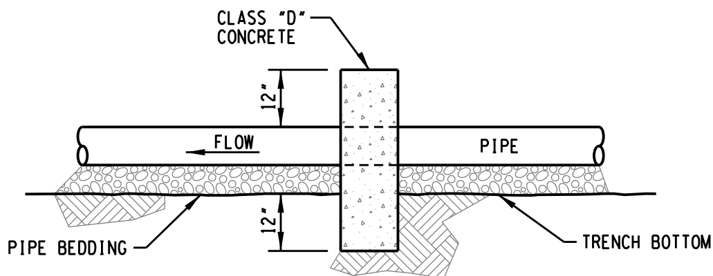
SECTION
