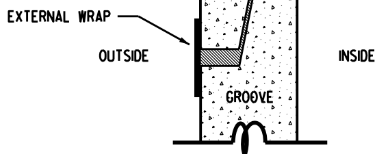
CLOSED JOINT
