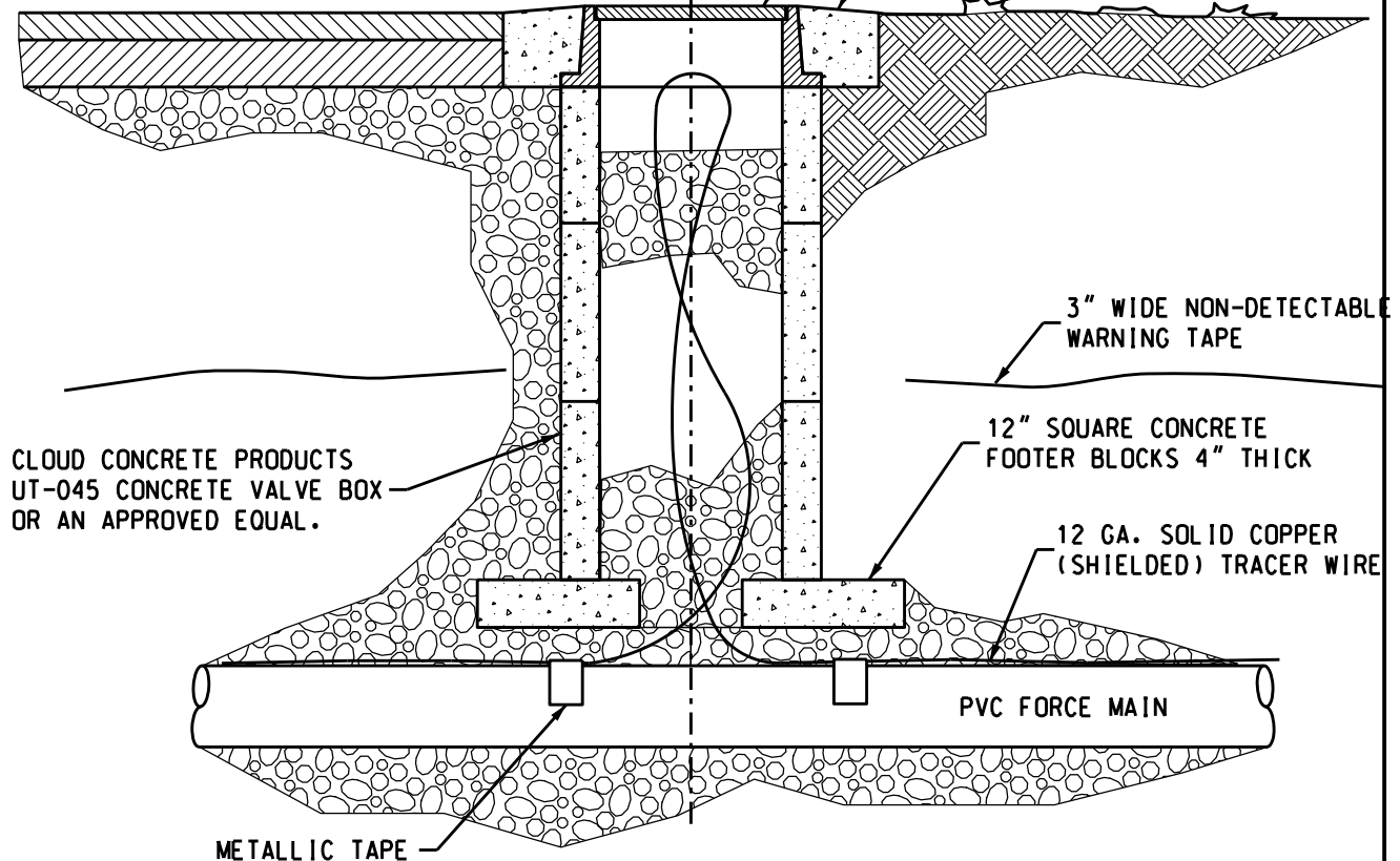
TRACER WIRE BOX DETAIL
