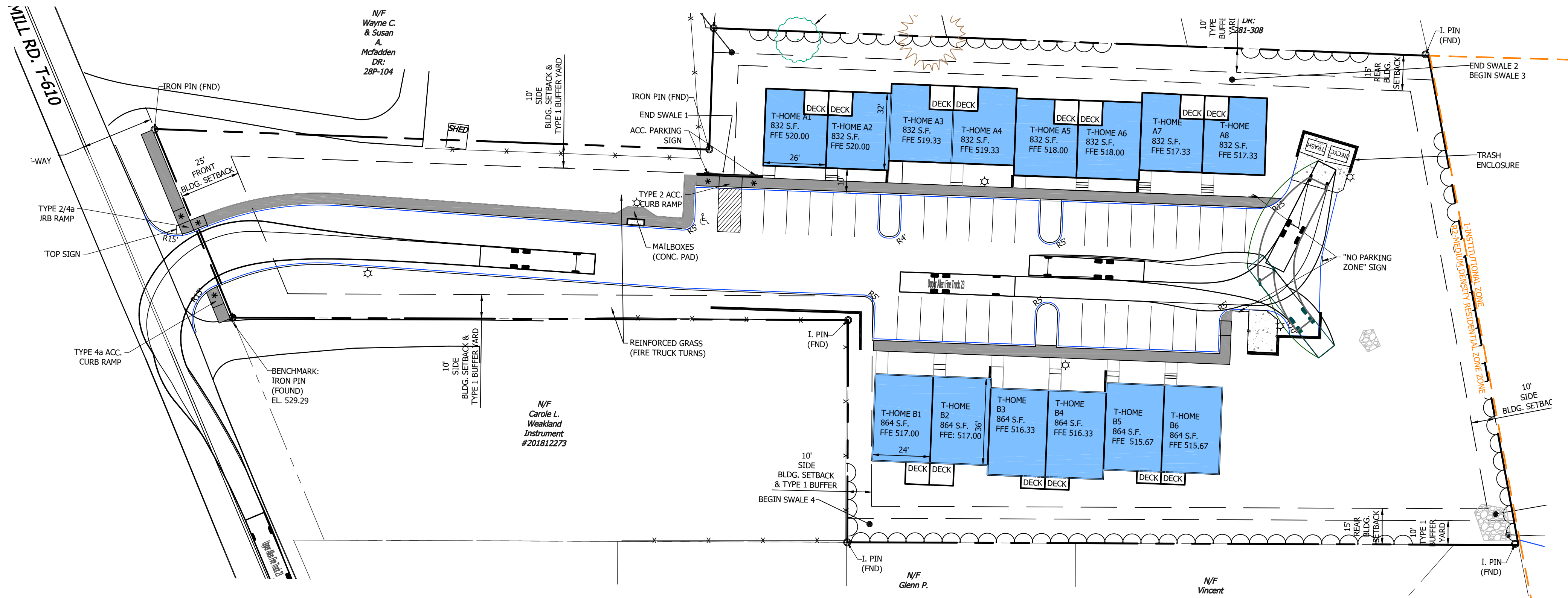
FIRE TRUCK TURNING
