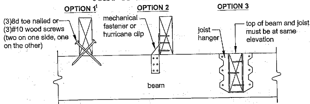
Figure 8 JOIST-TO-BEAM CONNECTIONS
