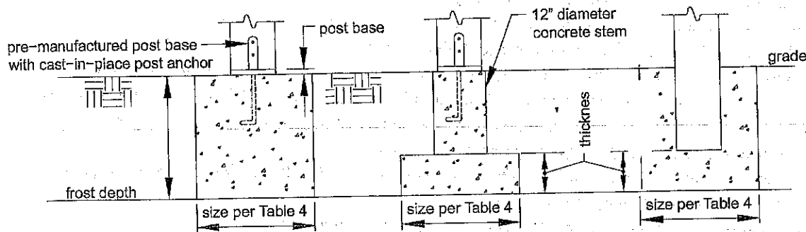
Figure 1 FOOTINGS
