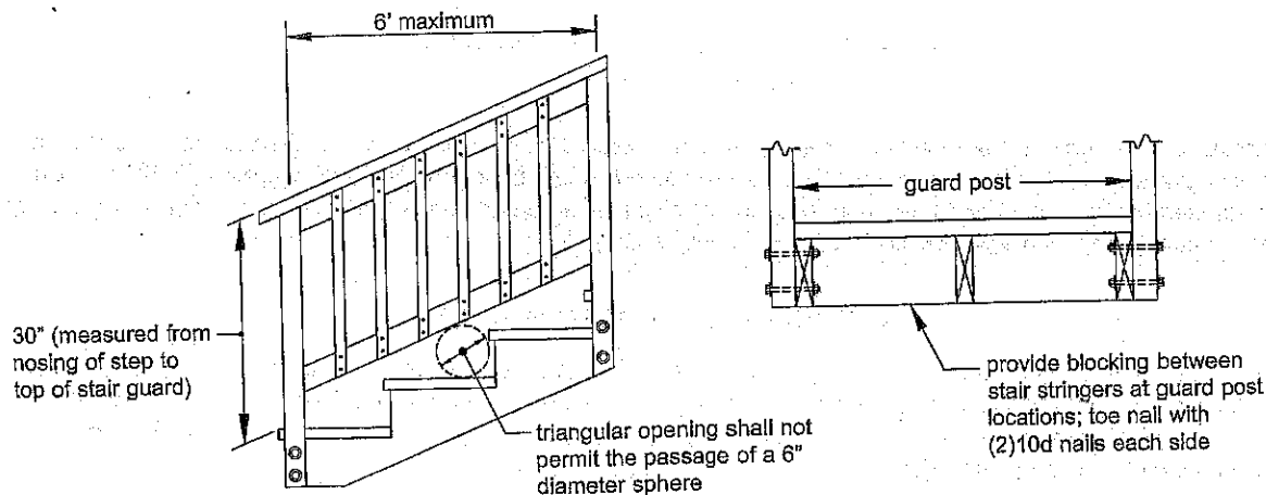
Figure 32 STAIR GUARDS
