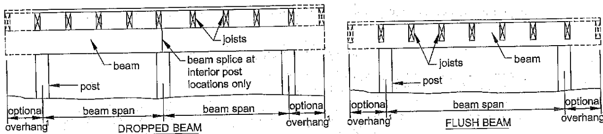
Figure 3 BEAM TYPES
