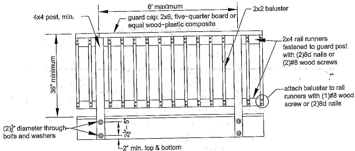
Figure 24 GUARDS
