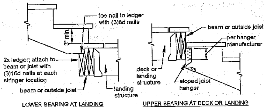
Figure 28 STRINGER BEARING
