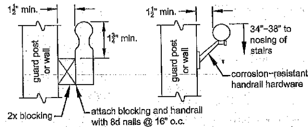
Figure 34 HANDRAIL GRASPABILITY
