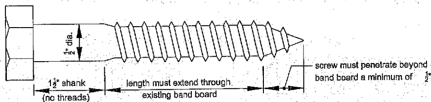
Figure 16 LAG SCREW
