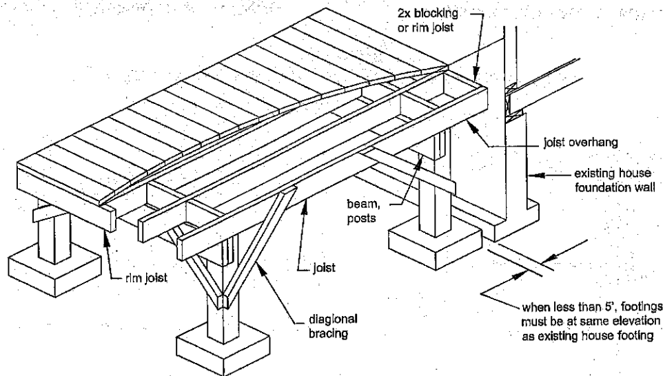
Figure 17 FREE-STANDING DECK
