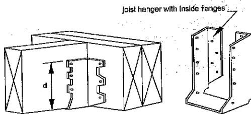
Figure 9 JOIST HANGERS
